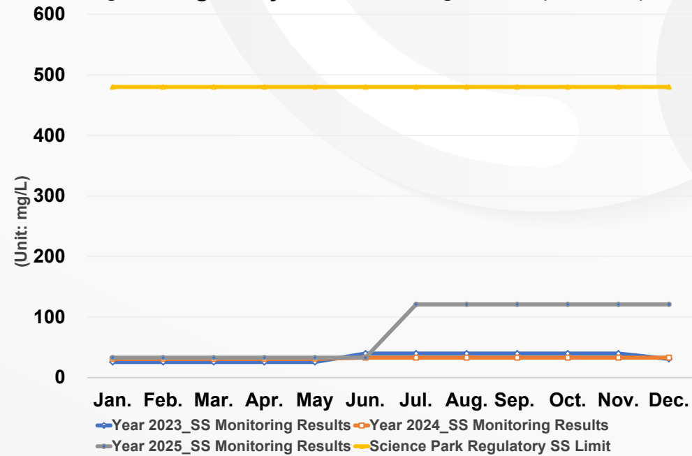
Suspended Solids (SS) Monitoring Results at Discharge Outlets in the Past Three Years
